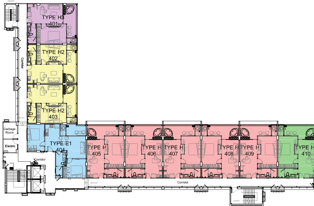
4th Floor Plan
